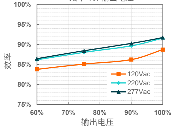
EUP-320S670SV( I_o=6700mA )
