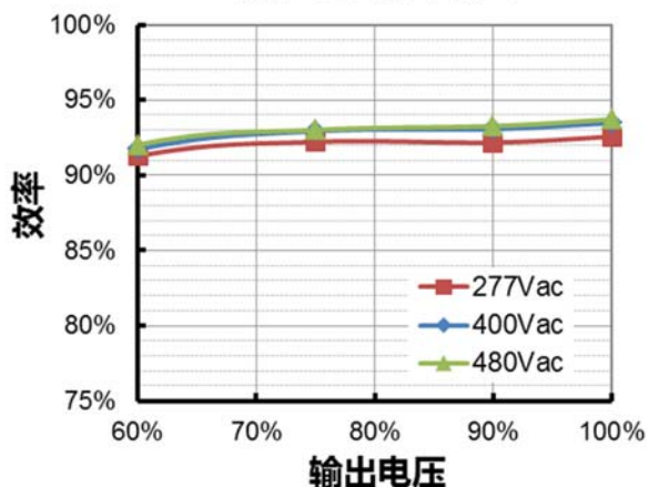
ESM-320S760Lx( I_o=5350mA ) 效率 vs. 输出电压
