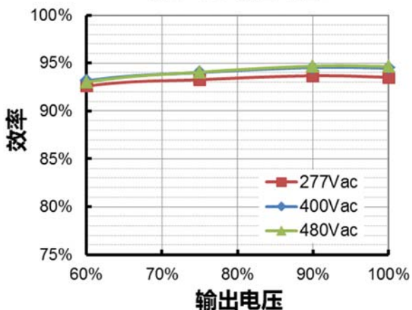
ESM-320S500Lx( I_o=2850mA ) 效率 vs. 输出电压
