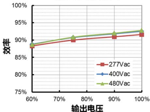
ESM-320S500Lx( I_o=5000mA ) 效率 vs. 输出电压
