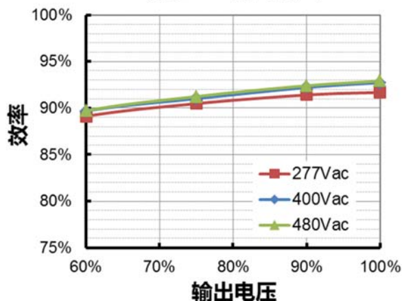
ESM-320S760Lx( I_o=7600mA ) 效率 vs. 输出电压
