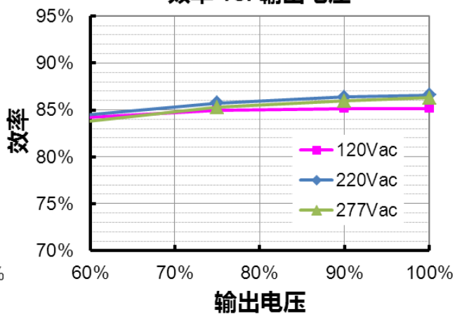
EUC-040S110DTM0005( I_o=860mA ) 效率 vs. 输出电压
