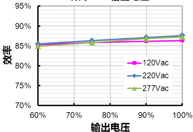
EUC-040S110DTM0001( I_o=1050mA ) 效率 vs. 输出电压
